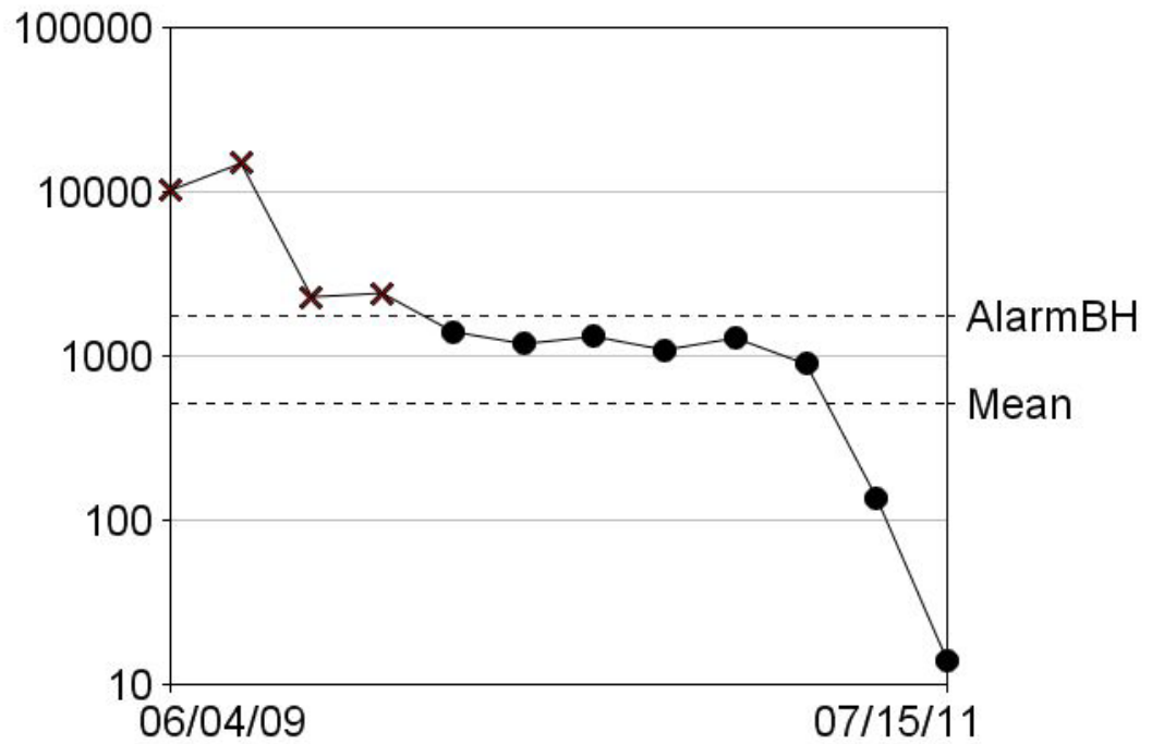
Wear Particle Trend
